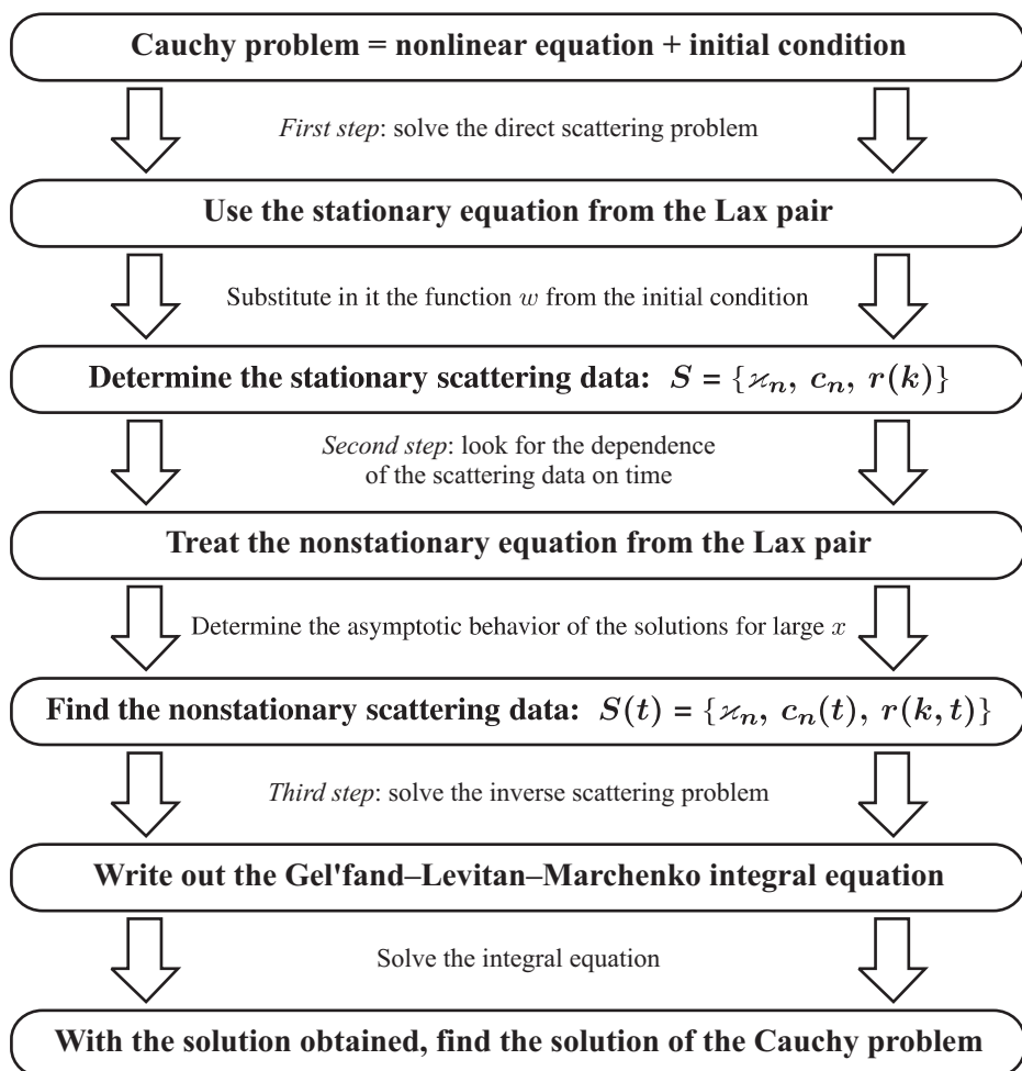
Figure 36.1. Main stages of solving the Cauchy problem for integrable nonlinear equations using the method of the inverse scattering problem.
