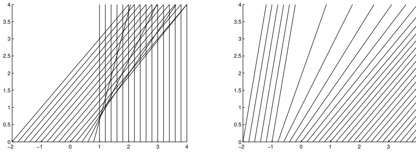
Figure 41.10. Burgers equation: characteristic curves for shock and rarefaction waves.
