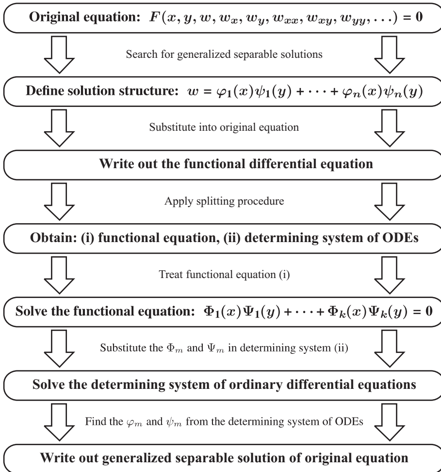
Figure 29.1. General scheme for constructing generalized separable solutions by the splitting method. Abbreviation: ODE stands for ordinary differential equation.
