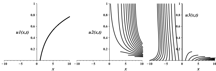
Figure 39.6. Solution u_1(x, t) for f(x) = 1 and solutions u_2(x, t) , u_3(x, t) for f(x) = x .
