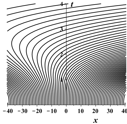
Figure 39.4. Characteristic curves for u_t + t^2 u u_x = 7 .
