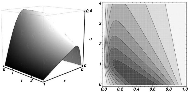
Figure 40.5. Numerical solution of the nonlinear diffusion equation: the 3D and contour plots for x \in [0, 1] and t \in [0, 4] .
