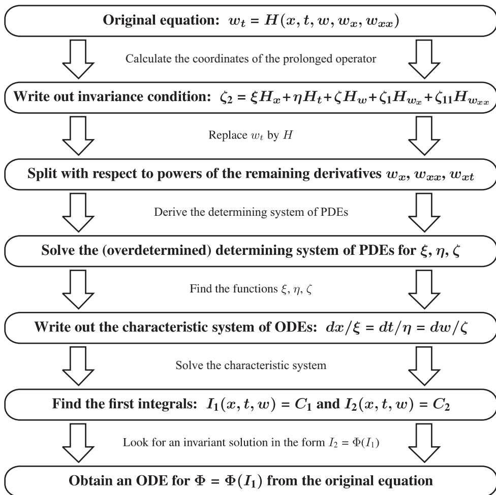
Figure 32.1. An algorithm for constructing invariant solutions for evolution second-order equations. Notation: ODE stands for ordinary differential equation and PDE stands for partial differential equation; \xi = \xi(x, t, w) , \eta = \eta(x, t, w) , \zeta = \zeta(x, t, w) ; \zeta_1, \zeta_2 , and \zeta_{11} are the coordinates of the prolonged operator, which are defined by formulas (32.1.3.2) and (32.1.3.7) with y = t .
