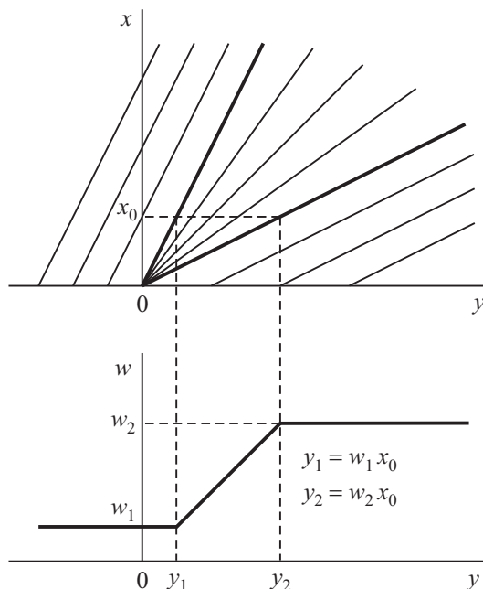
Figure 23.1. Characteristics of the Cauchy problem (23.2.2.3), (23.2.1.2) with the initial profile (23.2.2.10) and the dependence of the unknown w on the coordinate y for w_1 = \frac{1}{2} , w_2 = 2 , and x_0 = 1 .
