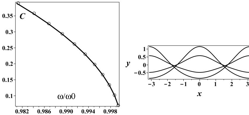
Figure 39.10. Frequency-amplitude dependence obtained numerically and asymptotically; surface profiles at times t = 0, \pi, \frac{5\pi}{3}, \frac{10\pi}{3} .
