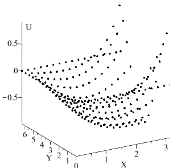
Figure 39.9. Numerical solution of the nonlinear Poisson equation.
