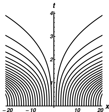
Figure 40.4. Characteristic curves for u_t + t^2 u u_x = 0 .
