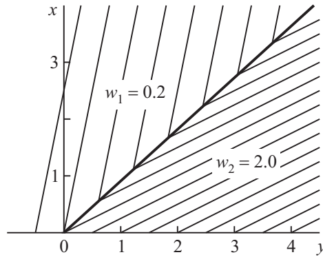
Figure 23.10. Characteristics and the discontinuity line for an unstable discontinuous solution (23.4.2.4).
