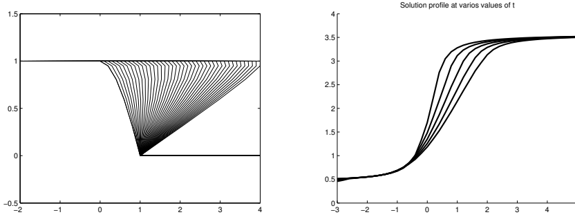
Figure 41.11. Burgers equation: shock and rarefaction waves.
