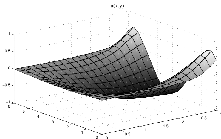
Figure 41.4. Surface plot of the solution of the nonlinear Poisson equation.
