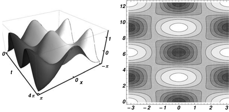
Figure 40.9. Numerical solution of the nonlinear standing waves problem: the 3D and contour plots for x \in [-n, \pi] and t \in [0, 4\pi] .
