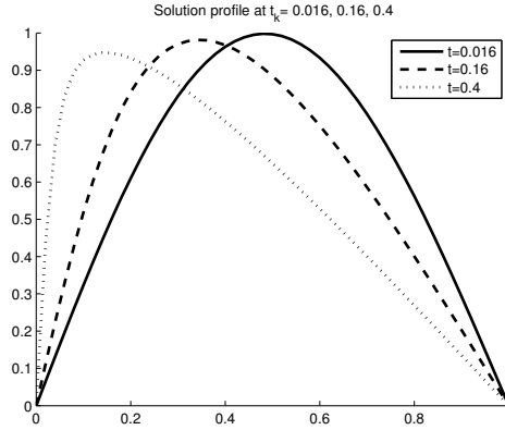
Figure 41.13. Burgers equation: solution profiles at t_k = 0.016, 0.16, 0.4 .
