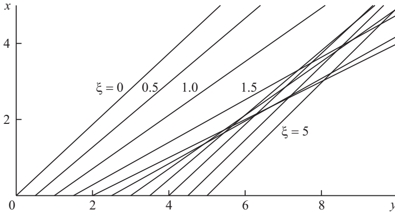
Figure 23.4. Characteristics for the Hopf's equation (23.2.2.3) with the initial profile (23.3.2.4).
