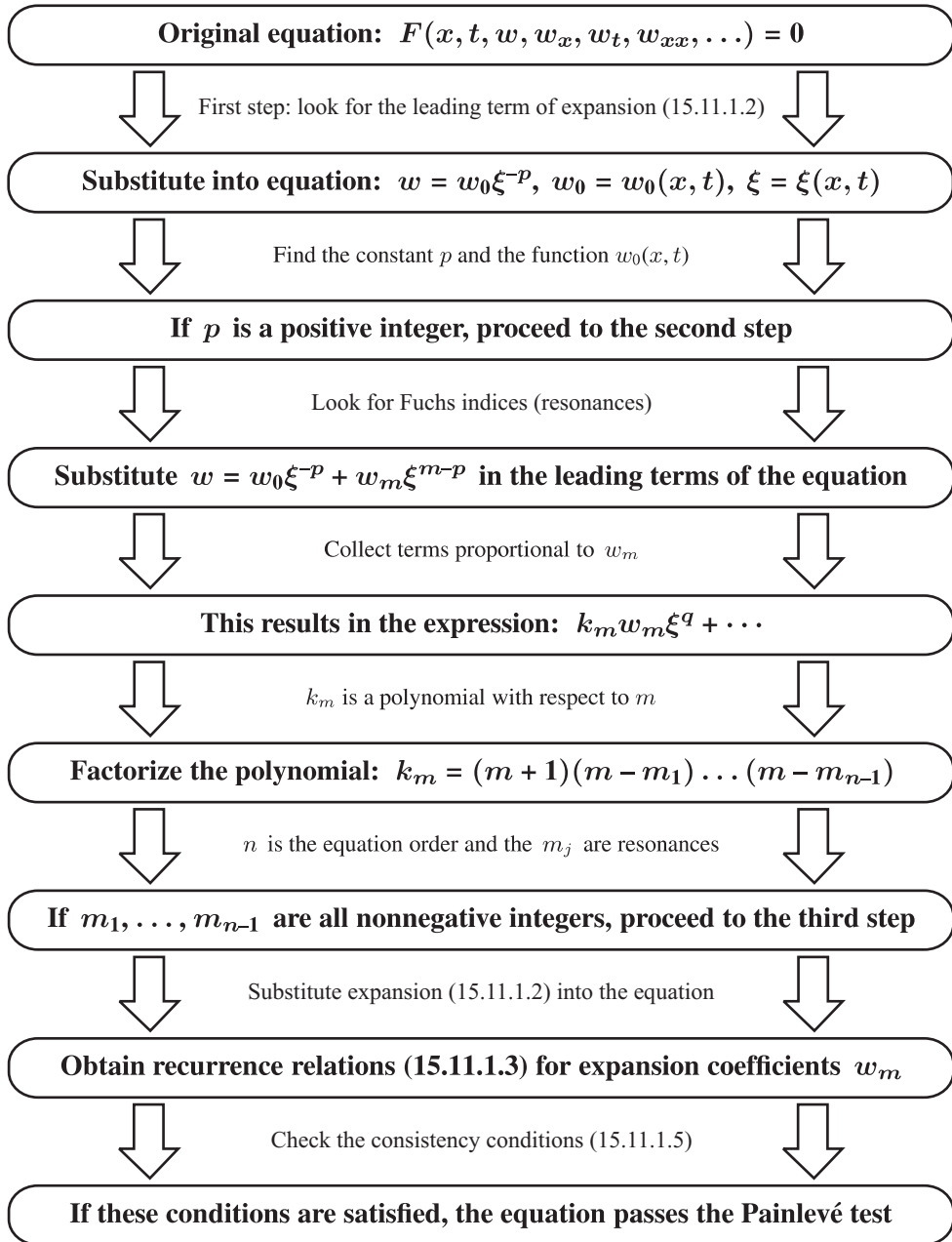
Figure 35.1. Basic steps of the Painlevé test for nonlinear equations of mathematical physics. It is assumed that \xi = x - x_0(t) for the simple scheme and \xi = \xi(x, t) for the general scheme.
