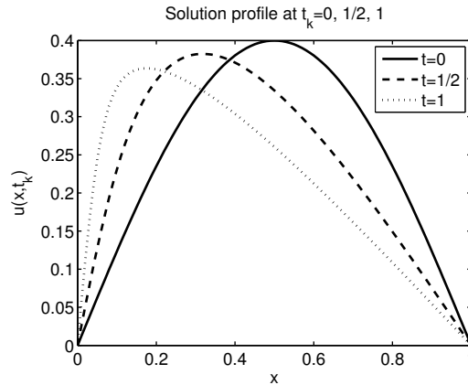
Figure 41.1. Surface profiles of the solution of the Burgers equation at t_k = 0, \frac{1}{2}, 1 .
