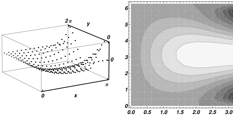
Figure 40.8. Numerical solution of the nonlinear Poisson equation: the 3D and contour plots inside the domain \mathcal{D} .
