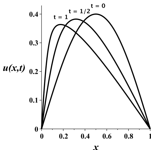
Figure 39.7. Numerical solution of the Burgers equation at t = 0, \frac{1}{2}, 1 .
