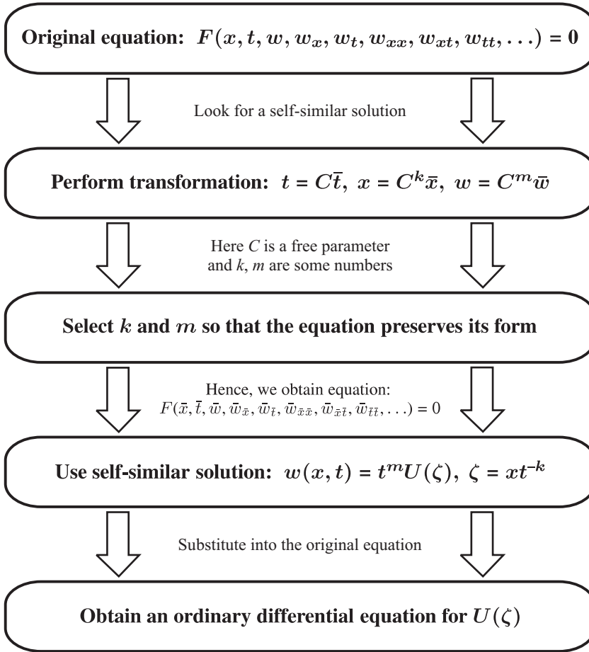
Figure 27.1. A simple scheme that is often used in practice for constructing self-similar solutions.
