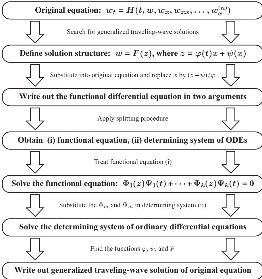
Figure 30.1. Algorithm for constructing generalized traveling-wave solutions for evolution equations. Abbreviation: ODE stands for ordinary differential equation.
