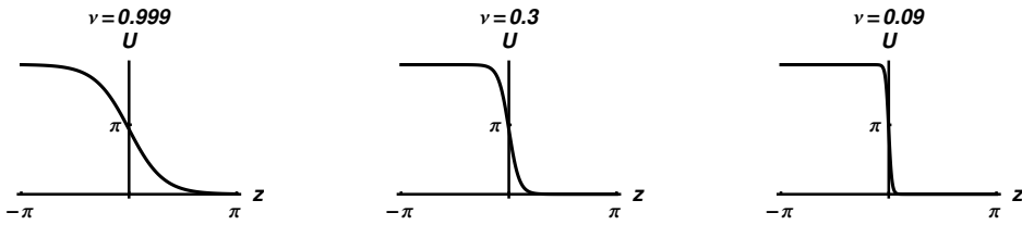
Figure 40.2. Traveling-wave solutions of the Burgers equation.
