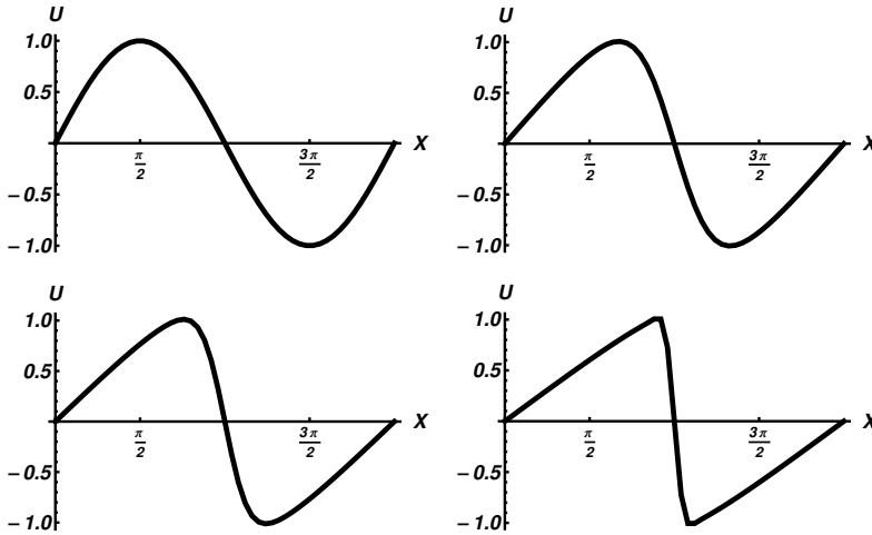
Figure 40.7. Inviscid Burgers equation: evolution of the wave profile for t = 0, 0.56, 0.84, 1.4 .
