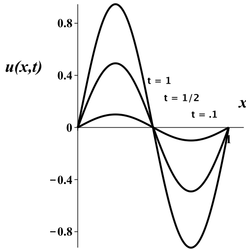
Figure 39.8. Numerical solution of the nonlinear wave equation at t = 0.1, 0.5, 1 .
