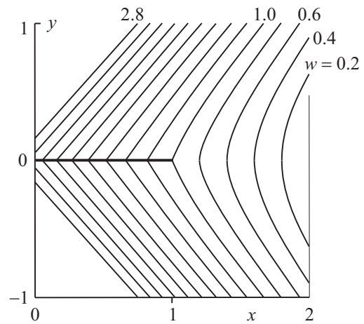
Figure 24.4. Level lines of the terminal value problem (24.3.6.1)–(24.3.6.2) for the Hamilton–Jacobi equation.
