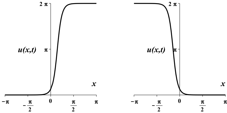
Figure 39.1. The kink and antikink solutions of the sine–Gordon equation.
