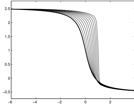
Figure 41.14. Numerical solution of inviscid Burgers equation.
