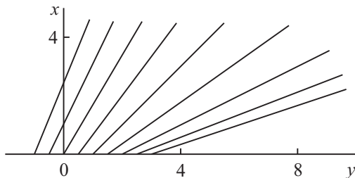
Figure 23.2. Characteristics for the Hopf's equation (23.2.2.3) with the initial profile (23.3.2.3).
