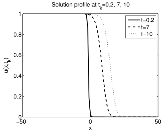
Figure 41.2. Surface profile evolution of the Fisher equation for t_k = 0.2, 7, 10 .
