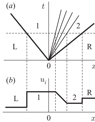
Figure 38.2. Solution for the Riemann problem: (a) centered waves in the (x, t) plane; (b) the u_i profile.
