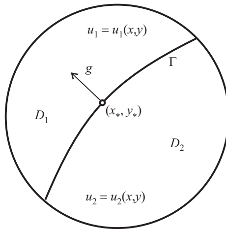
Figure 24.1. Generalized viscosity solution undergoes a discontinuity along the singular curve \Gamma ; the solution is smooth in the subdomains D_1 and D_2 .
