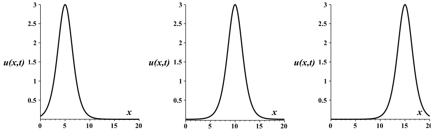
Figure 39.2. The traveling-wave solution of the Korteweg-de Vries equation.
