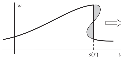
Figure 23.6. Replacement of the many-valued part of the wave profile by a discontinuity that cuts off domains with equal areas (shaded) from the profile of a breaking wave.
