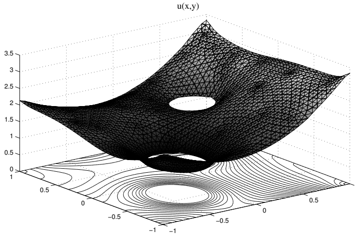
Figure 41.8. Mesh plot with the contour lines of the solution of the Poisson–Boltzmann equation.
