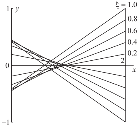
Figure 24.3. Characteristics of the terminal value problem (24.3.6.1)–(24.3.6.2) for the Hamilton–Jacobi equation.
