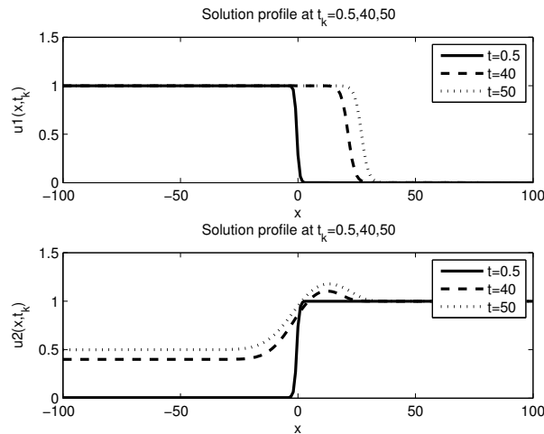
Figure 41.3. Surface profiles of the solution at t_k = 0.5, 40, 50 .
