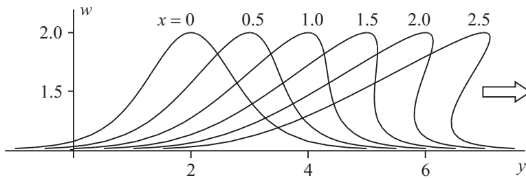
Figure 23.5. The evolution of a solitary wave for the Hopf's equation (23.2.2.3) with the initial profile (23.3.2.4).
