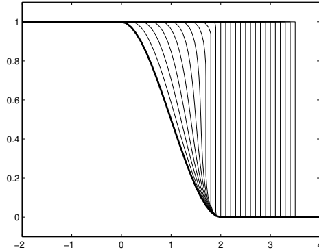
Figure 41.12. Burgers equation: formation of shock waves.
