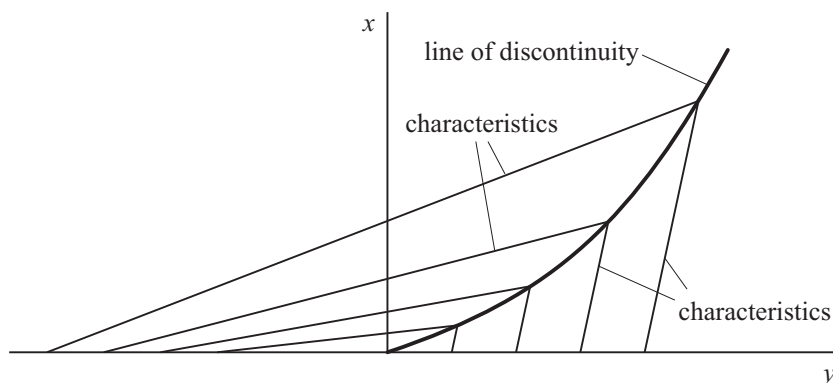
Figure 23.7. Mutual arrangement of characteristics and lines of discontinuity in the case of a stable shock wave.
