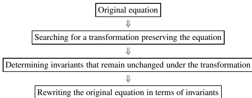
Figure 28.1. General scheme of using invariants for solving mathematical equations.
