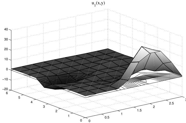
Figure 41.6. Surface plot with contour lines of the solution u_1(x, y) .
