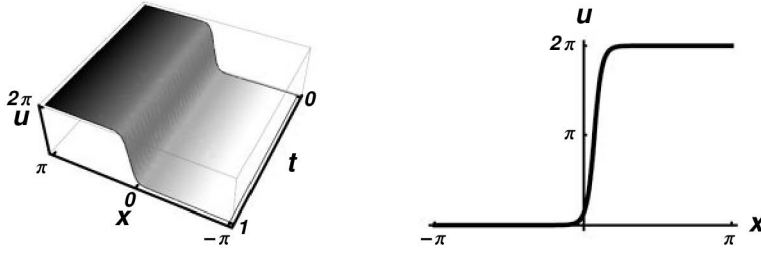
Figure 40.1. The kink solution of the sine-Gordon equation in 3D and 2D spaces.
