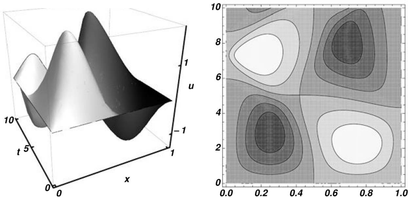
Figure 40.6. Numerical solution of the nonlinear wave equation: the 3D and contour plots for x \in [0, 1] and t \in [0, 10] .
