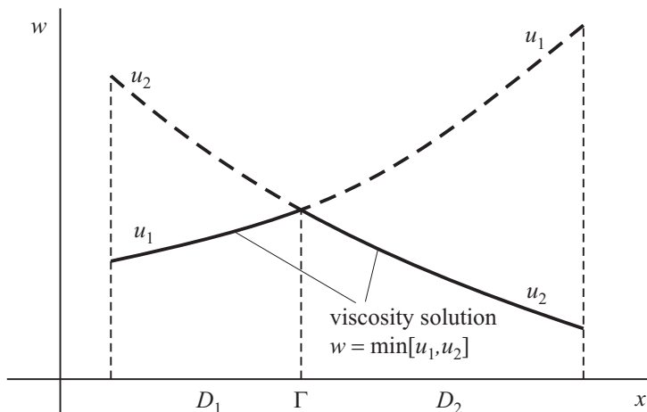
Figure 24.2. Graphic construction of a generalized viscosity solution by joining together smooth solutions.
