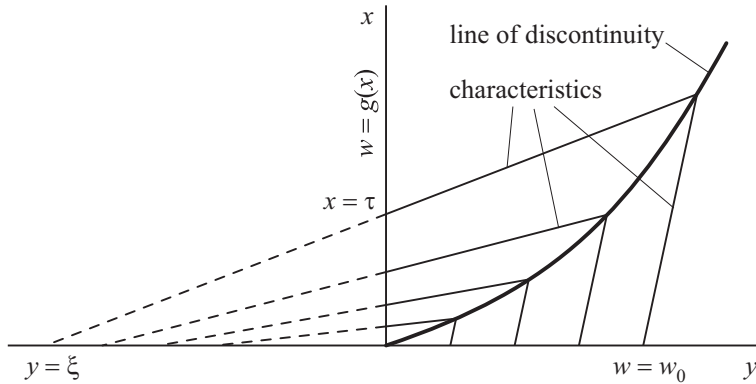
Figure 23.9. Characteristics of the problem of propagation of a signal.
