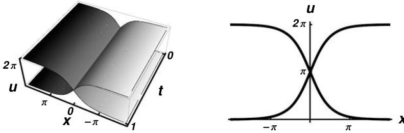
Figure 40.3. The kink and antikink solutions of the SG equation in 3D and 2D spaces.
