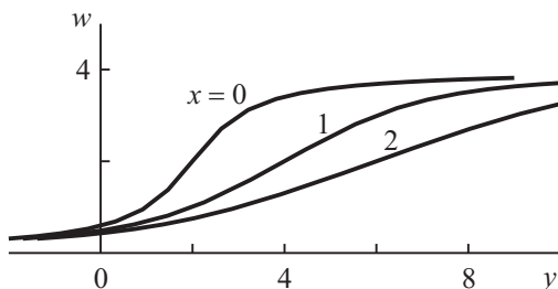
Figure 23.3. The evolution of a rarefaction wave for the Hopf's equation (23.2.2.3) with the initial profile (23.3.2.3).
