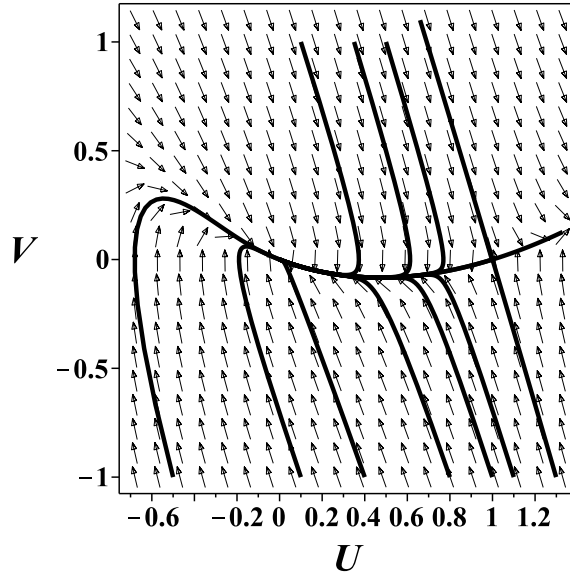
Figure 39.3. The phase portrait on the plane (U, V) for the Fisher equation.
