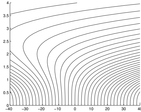
Figure 41.9. Characteristic curves for u_t + t^2 u u_x = 7 .
