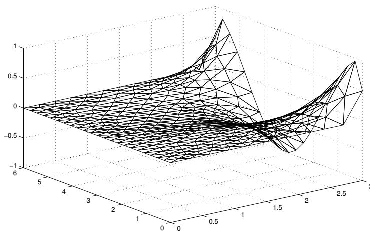
Figure 41.5. Mesh plot for the solution of the nonlinear Poisson equation.
