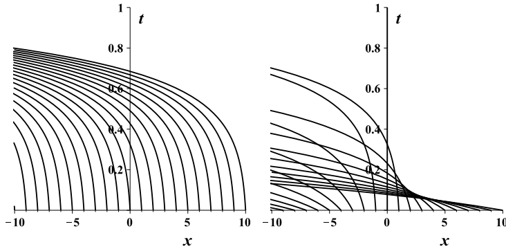
Figure 39.5. Characteristic curves for f(x) = 1 and f(x) = x .
