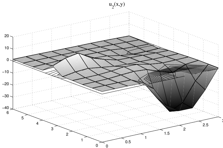
Figure 41.7. Surface plot with contour lines of the solution u_2(x,y) .
