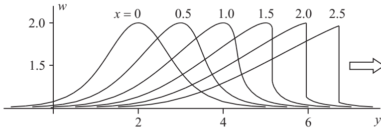
Figure 23.8. The formation of a shock wave generated from a solitary wave with the smooth initial profile.
