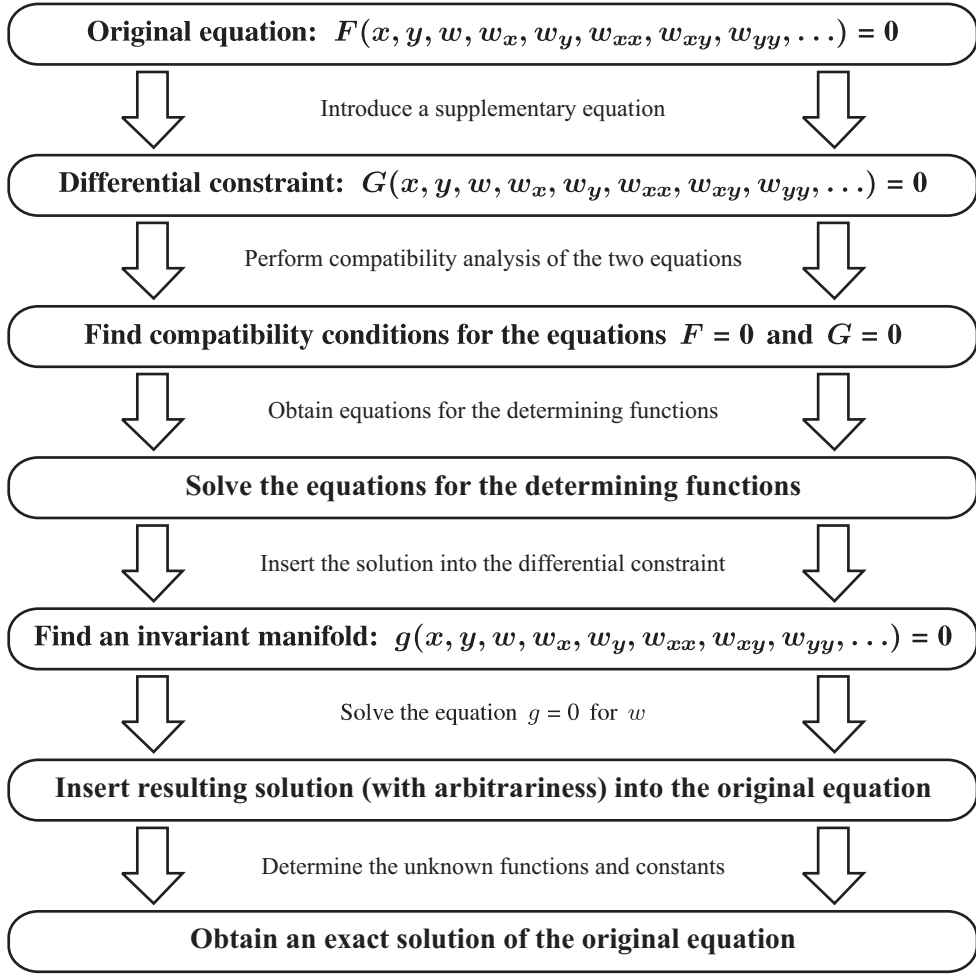
Figure 34.1. Algorithm for the construction of exact solutions by the method of differential constraints.
