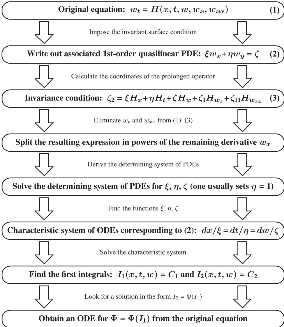
Figure 33.1. Algorithm for the construction of exact solutions by a nonclassical method for second-order evolution equations. Here, ODE stands for ordinary differential equation and PDE for partial differential equation.
